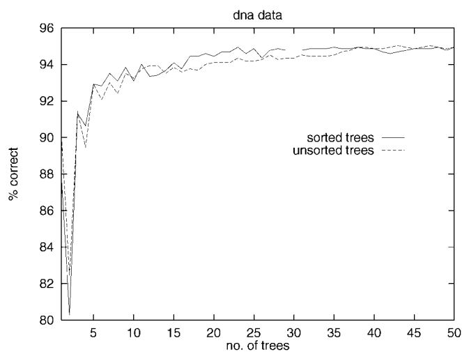
Fig. 6. Comparison of test set accuracies between forests with sorted and unsorted trees.
