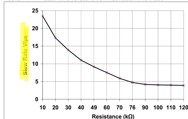
FIGURE 1-1: SLEW RATE VS. SLOPE-CONTROL RESISTANCE VALUE
