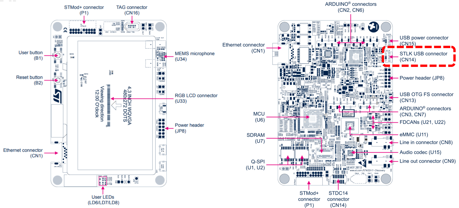
Figure 5. STM32H745I-DISCO and STM32H750B-DK Discovery board bottom layout
