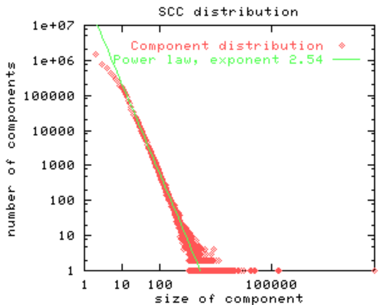
Figures 5 and 6: Distribution of weakly connected components and strongly connected components on the web. The sizes of these components also follow a power law.
