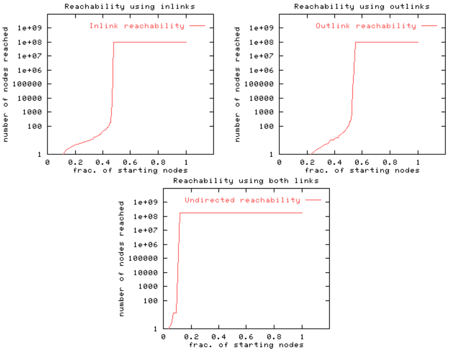
Figure 7: Cumulative distribution on the number of nodes reached when BFS is started from a random node. Figure (a) follows in-links, (b) follows out-links, and (c) follows both in and out links. Notice that there are two distinct regions of growth, one at the beginning and an "explosion" in 50 % of the start nodes in the case of in- and out-links, and for 90% of the nodes in the undirected case. These experiments form the basis of our structural analysis.
