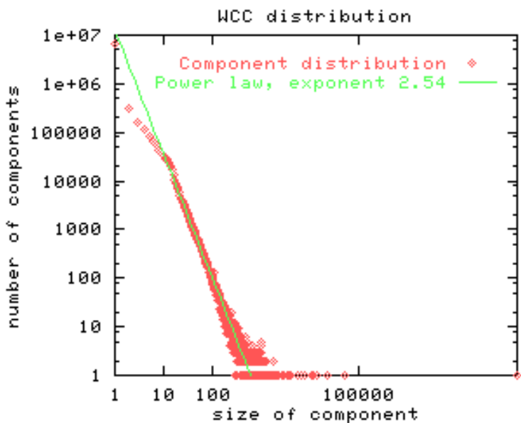
Figures 5 and 6: Distribution of weakly connected components and strongly connected components on the web. The sizes of these components also follow a power law.
