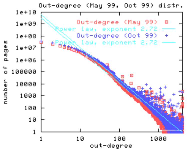
Figures 3 and 4: In- and out-degree distributions show a remarkable similarity over two crawls, run in May and October 1999. Each crawl counts well over 1 billion distinct edges of the web graph.
