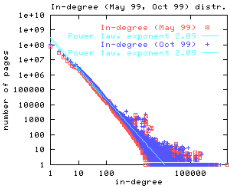
Figures 3 and 4: In- and out-degree distributions show a remarkable similarity over two crawls, run in May and October 1999. Each crawl counts well over 1 billion distinct edges of the web graph.
