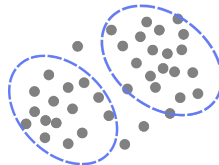
unsupervised learning
