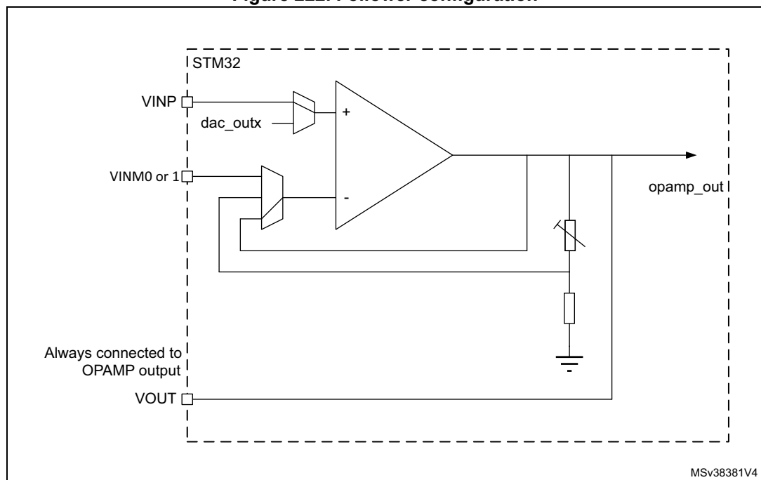
Figure 222. Follower configuration
