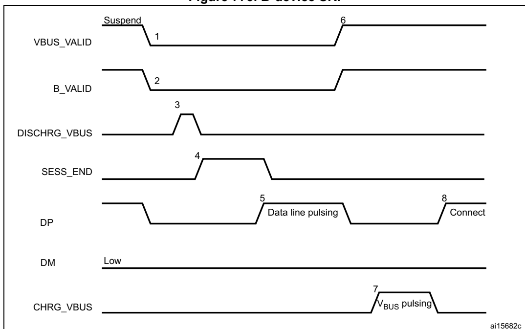
Figure 773. B-device SRP
