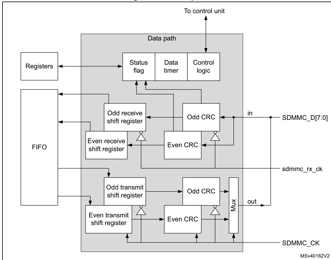
Figure 706. Data path
