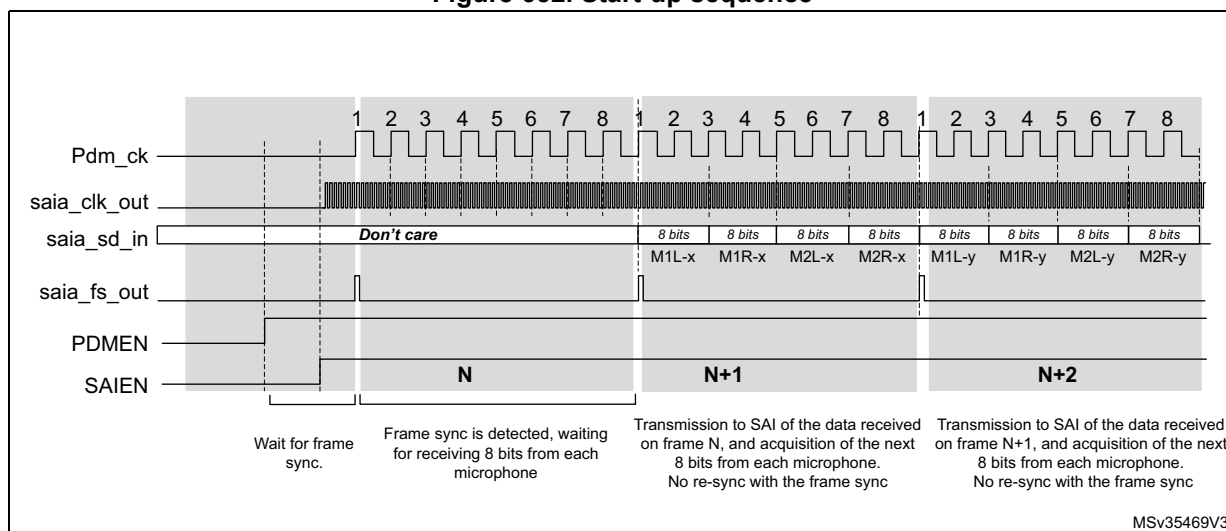
Figure 652. Start-up sequence
