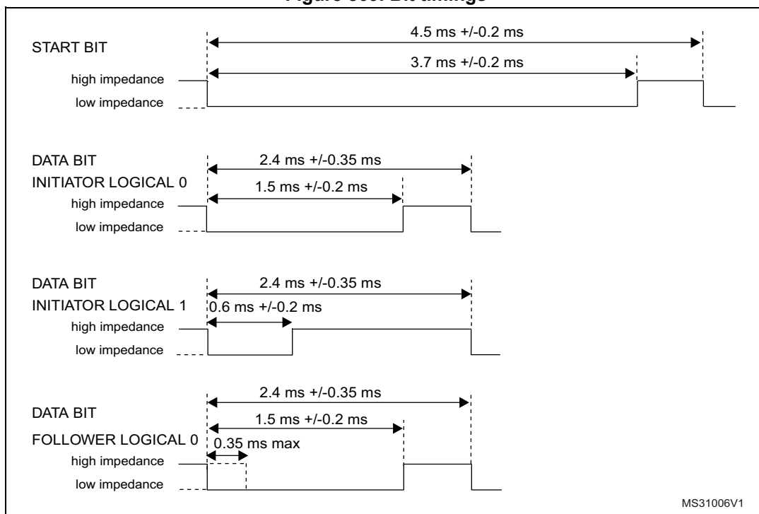
Figure 809. Bit timings
