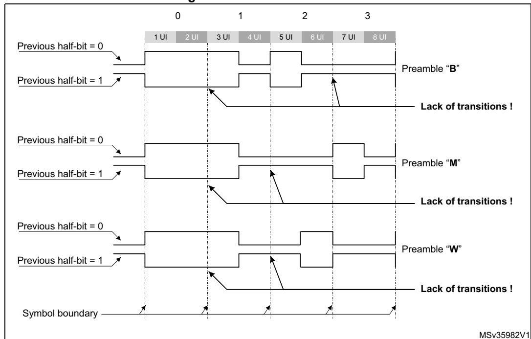
Figure 668. S/PDIF Preambles
