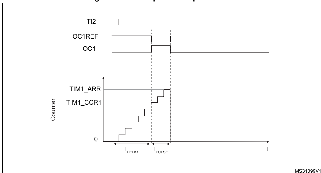
Figure 473. Example of one pulse mode.
