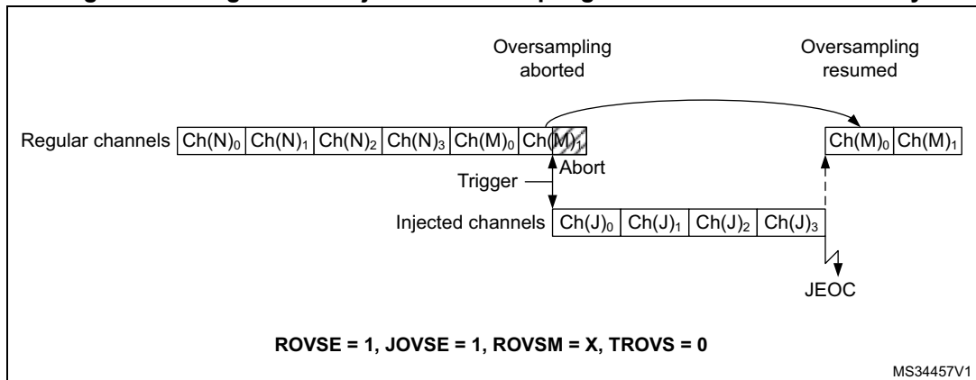
Figure 185. Regular and injected oversampling modes used simultaneously
