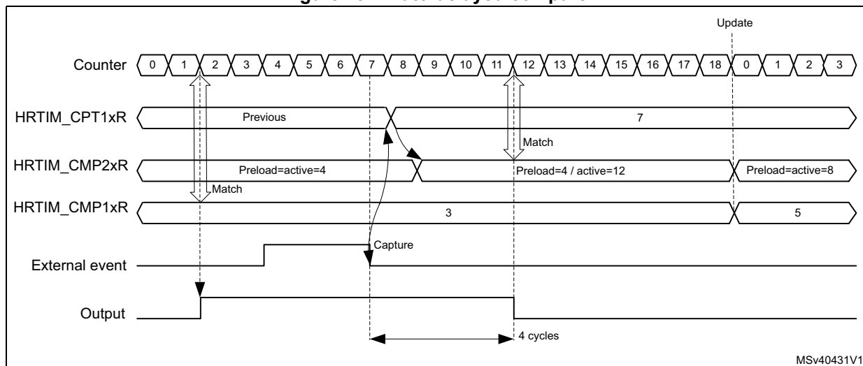
Figure 291. Auto-delayed compare
