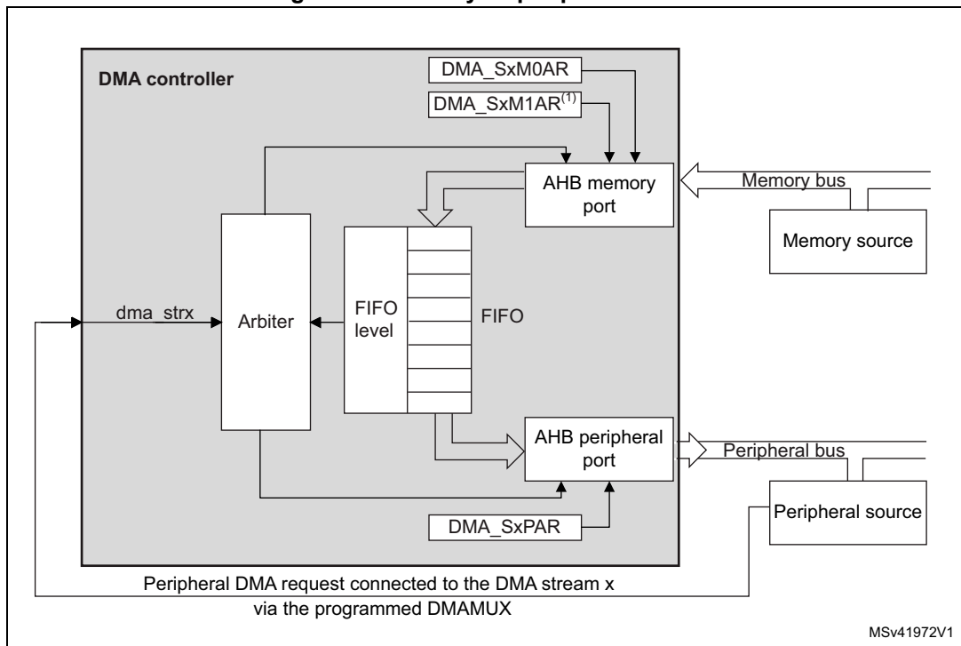
Figure 80. Memory-to-peripheral mode
