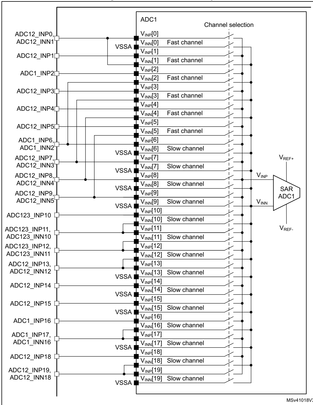
Figure 138. ADC1 connectivity
