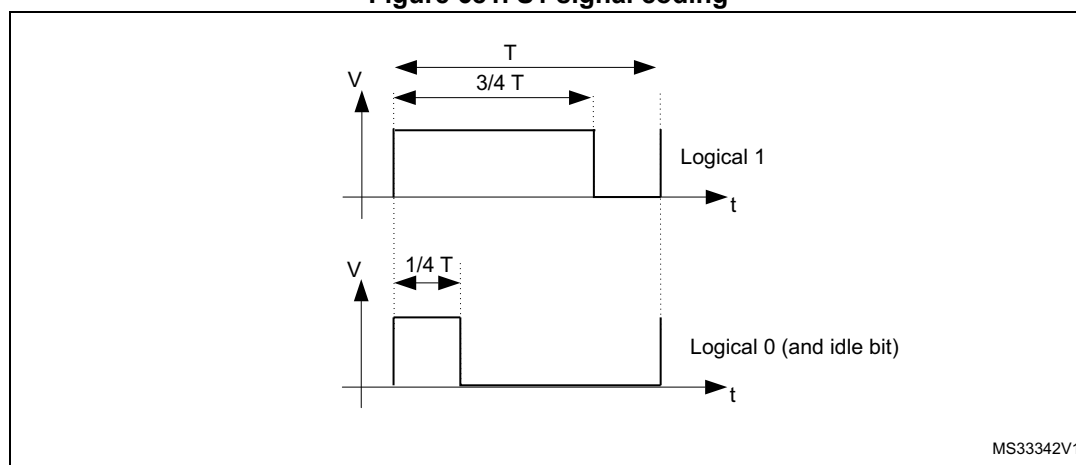
Figure 681. S1 signal coding
