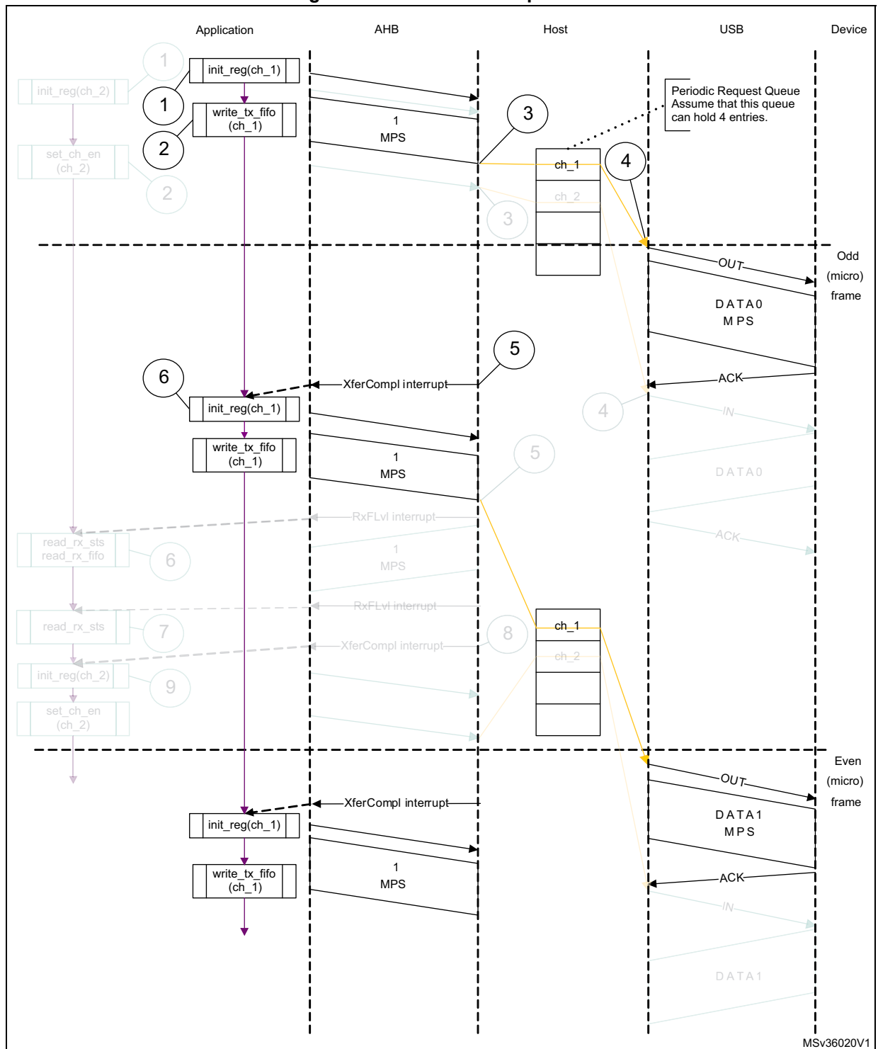
Figure 758. Normal interrupt OUT
