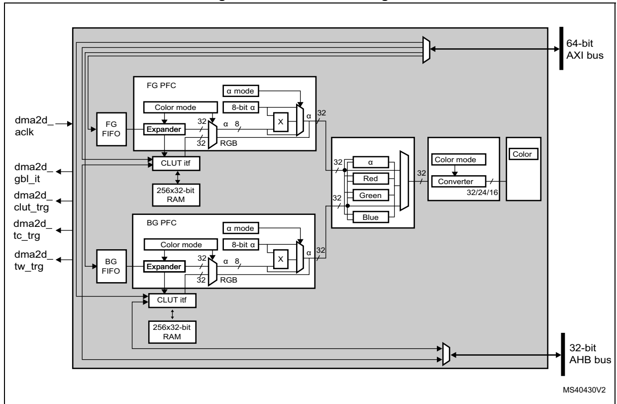
Figure 87. DMA2D block diagram
