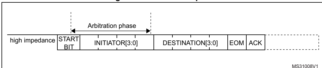
Figure 811. Arbitration phase
