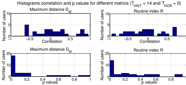
Figure 5: Histograms of the correlation and of the p-values for T_{HIST} = 14 day.
